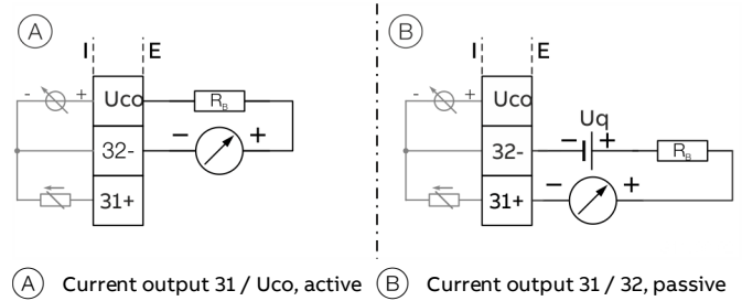
Figure 23: (I = internal, E = external, RB = load)
