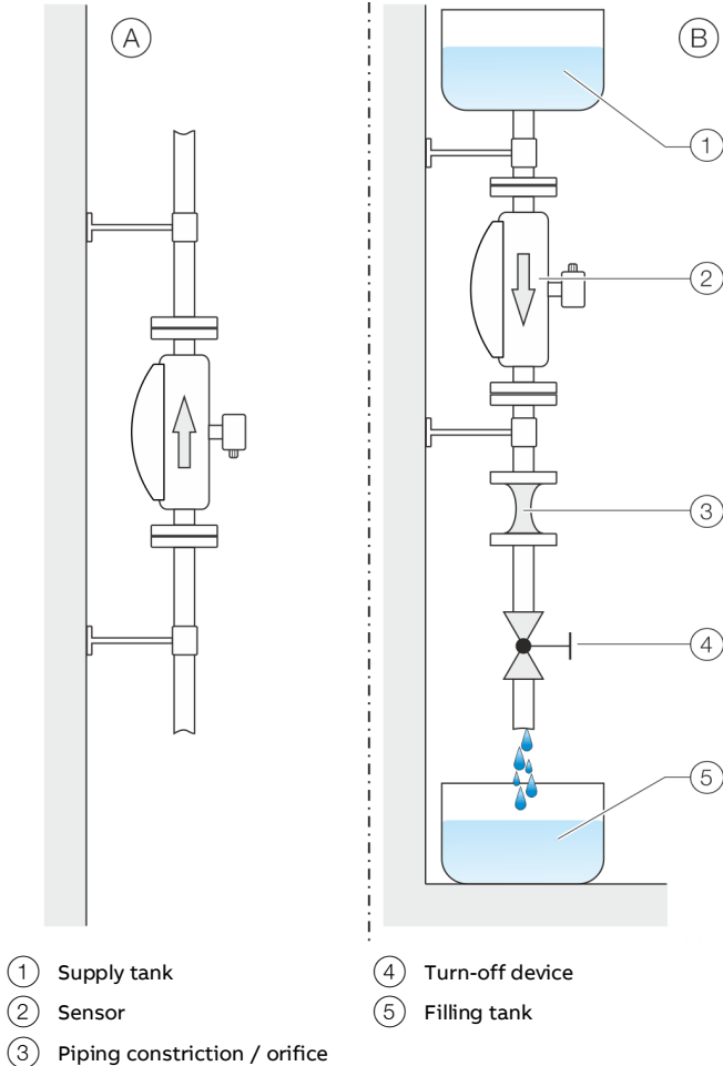
Figure 4: Vertical installation
