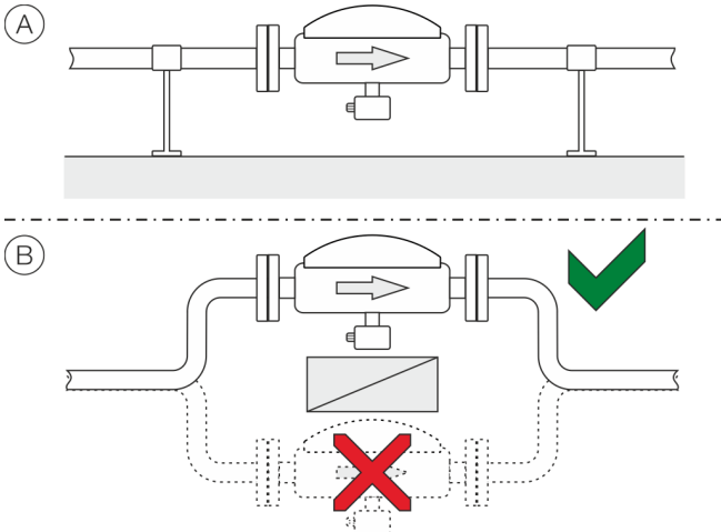
Figure 6: Horizontal installation
